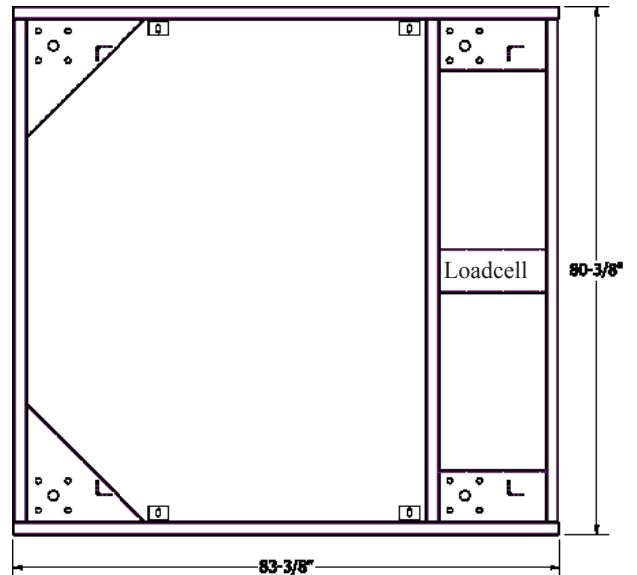
Frame Dimensions
